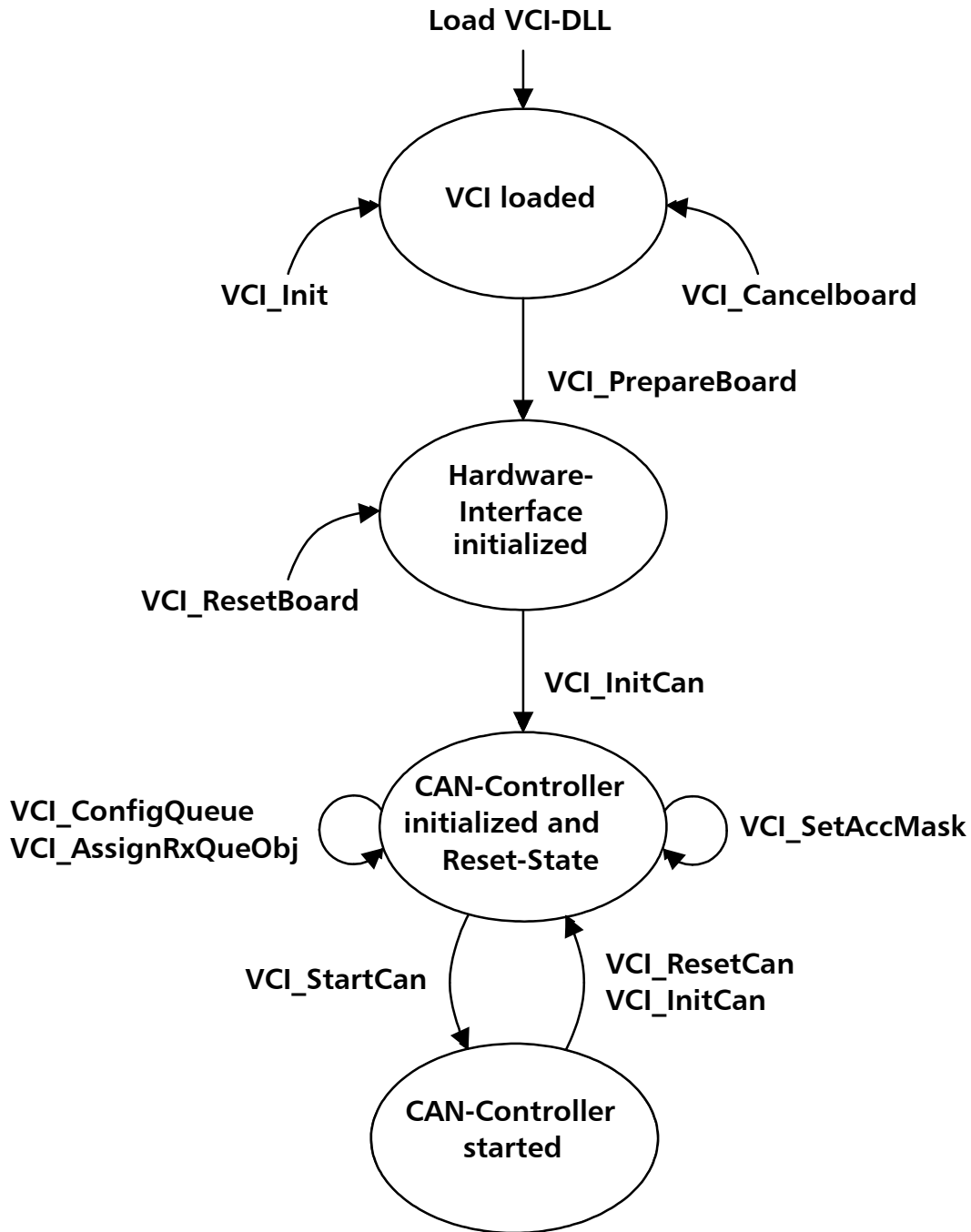
Fig. 2 - 1 State Diagram for Board Initialization
