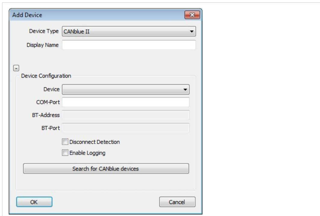
Fig. 5 Add Device
