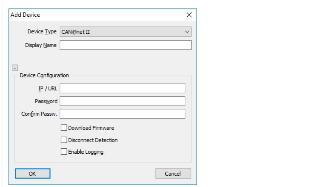
Fig. 8 Add Device
