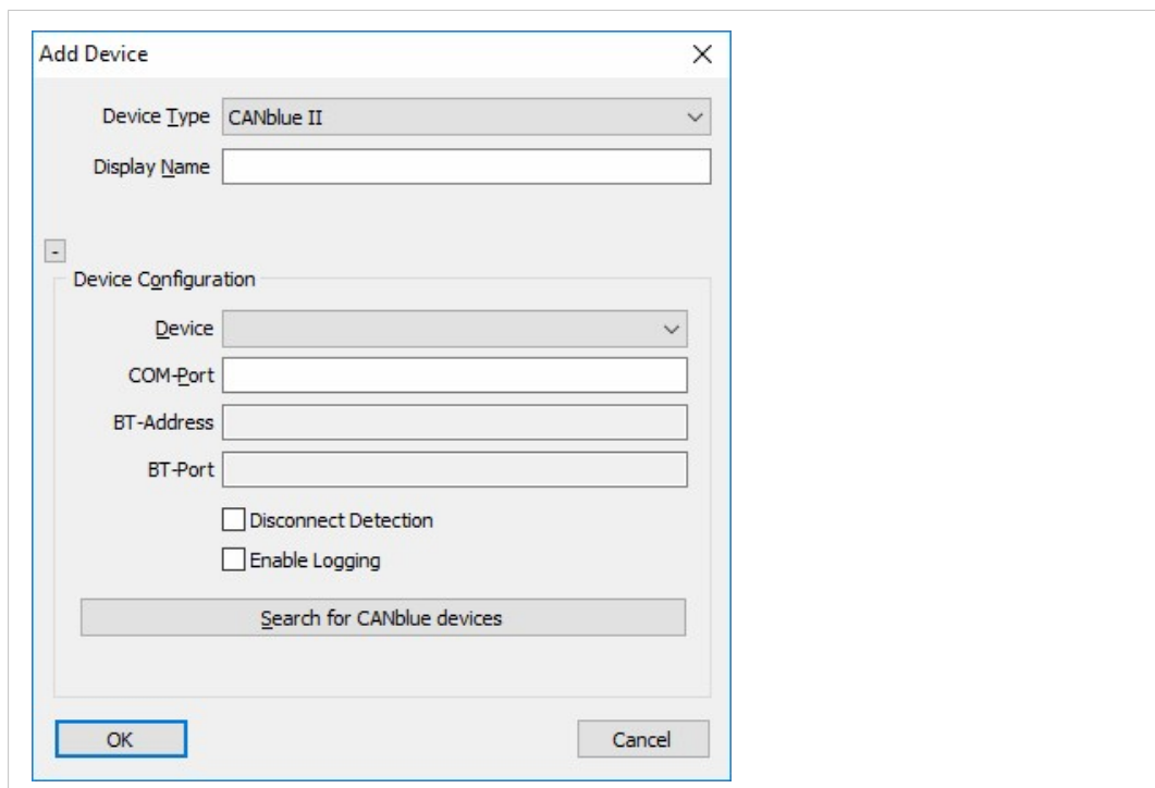
Fig. 11 Add Device
