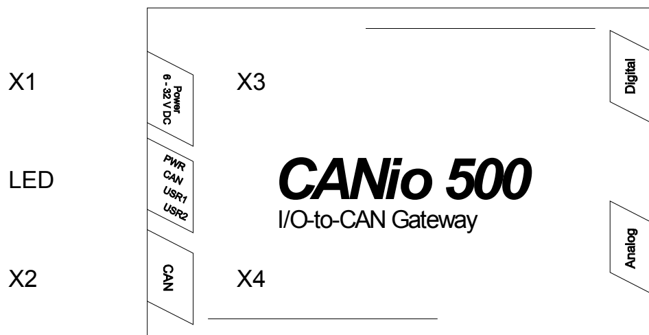
Figure 2-1: Connector assignments
