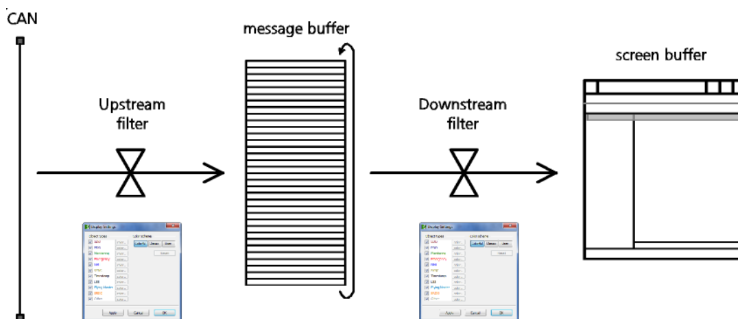
Figure 3.12: Idea of reception filtering
