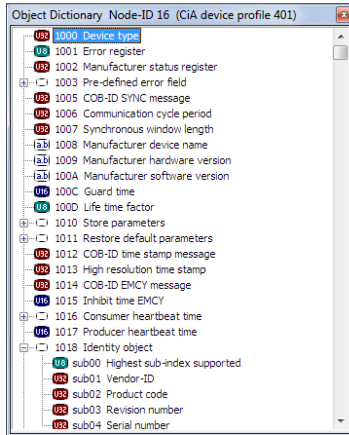
Figure 3.5: Readout of an Object Dictionary
