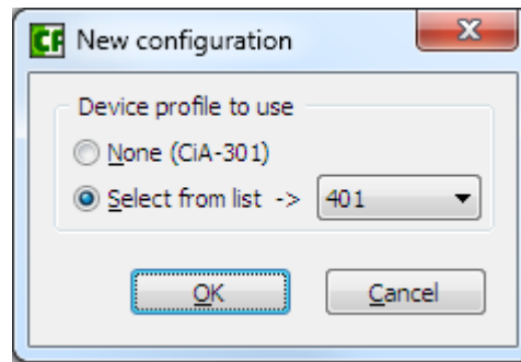
Figure 3.7: Create new configuration
