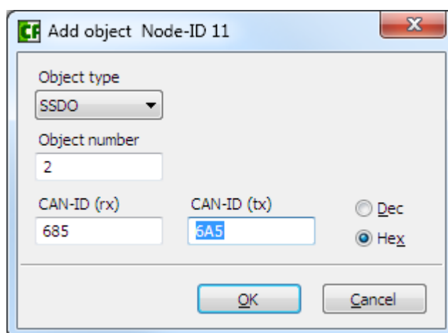
Figure 3.8: Add CANopen communication object (e.g. SDO)
