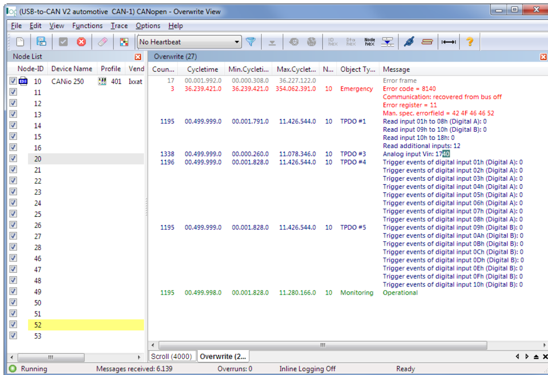
Figure 3.1: Overwrite View
